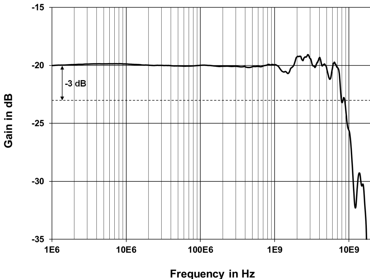
Fig. 4-2: Amplitude frequency response of the R&S RT-ZS60
