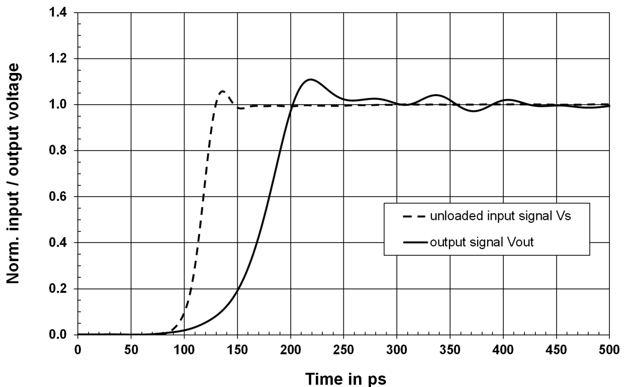
Fig. 4-3: Step response of the R&S RT-ZS60
