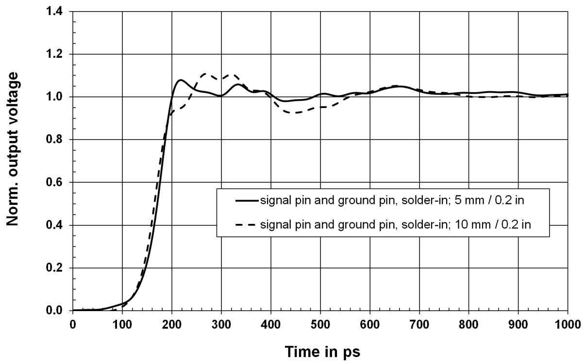
Fig. 4-6: Step response of the R&S RT-ZS60 with a type 2 connection
