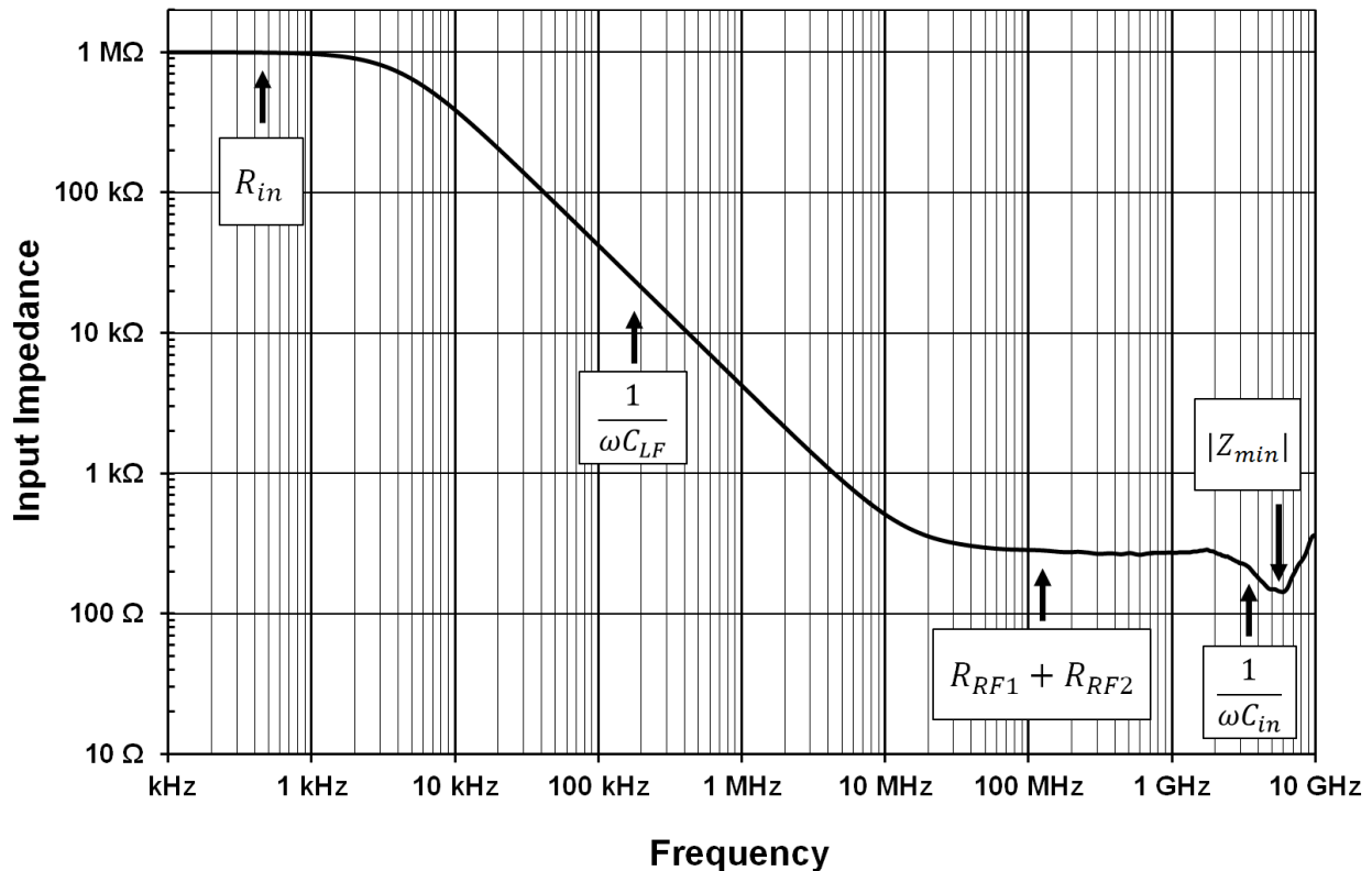
Fig. 4-8: Magnitude of the input impedance of the R&S RT-ZS60 probe as a function of frequency
