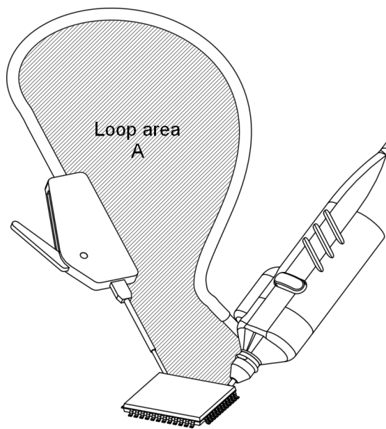
Fig. 4-4: Ground connection and connection inductance
