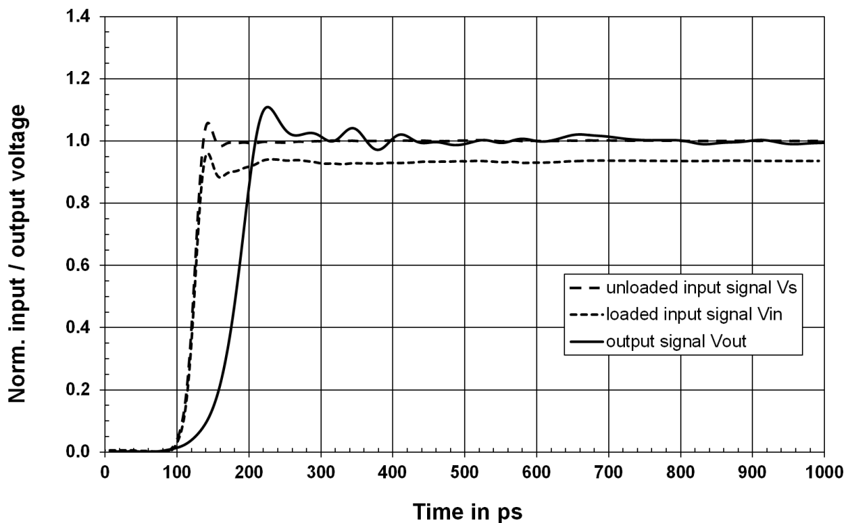
Fig. 4-10: Unloaded and loaded input signal and step response using the example of R&S RT-ZS60
